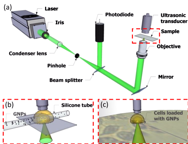
Fig. 1 (a) Representation of the photoacoustic microscopy (PAM) system. (b) Representation of the setup for the phantom experiment. The sample and ultrasound transducer were immersed in water. (c) Representation of the setup for the cell experiment. The cells grew on the bottom of a petri dish and were immersed in phenol red-free culture medium.
