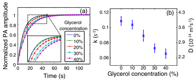
Fig. 3 (a) Photoacoustic recovery after photothermal bleaching (PRAP) in glycerol aqueous solutions with different concentrations. (b) Recovery rate and diffusion coefficient in each solution. Error bars show 95% confidence bounds.
