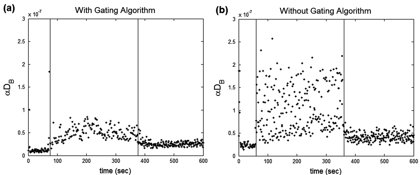
Fig. 3 (a), Raw DCS signal ( \alpha D_B ) acquired during exercise with application of gating algorithm. (b), Raw DCS signal acquired during exercise without application of gating algorithm. Exercise was performed at 25% MVC, with 1-s contraction/relaxation. The bold vertical lines denote beginning and end of exercise.
