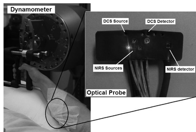
Fig. 1 Experimental setup showing dynamometer and flexible fiber-optic probe containing source and detector fibers for both NIRS and DCS, taped to forearm flexor muscles (flexor digitorum superficialis/profundus). Subject is supine, while arm is slightly elevated on a pillow. Hand is resting around handgrip attachment of the dynamometer.
