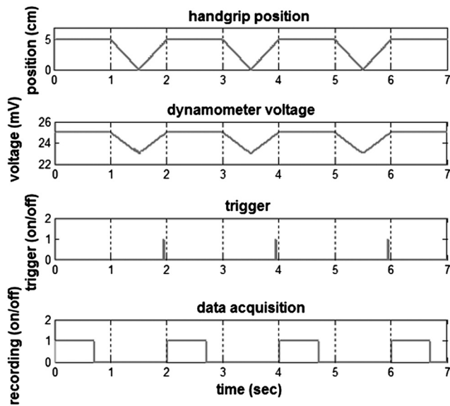
Fig. 2 Input and control signals for the gating algorithm controlling data acquisition during exercise. The dynamometer voltage is the input signal, which parallels the handgrip position. A handgrip position of 0 cm corresponds to fully contracted, whereas 5 cm corresponds to fully relaxed (no motion). The trigger signal is high following the rising edge of the dynamometer voltage. The delay between the trigger impulse and the beginning of data recording accounts for residual muscle motion once the dynamometer voltage has surpassed the threshold.
