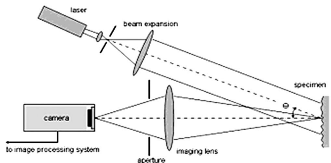
Fig. 3 Experimental system.
