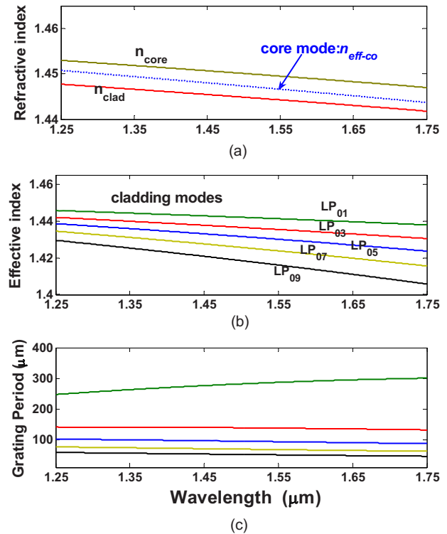
Fig. 1 (a) Refractive indices of core and cladding of the fiber; the dotted line is the effective index of the guided core mode. (b) The effective indices of the first five odd-cladding modes (LP 0m , m = 1, 3, 5, \dots ) of the proposed fiber device. (c) The phase-matching grating periods versus the coupling wavelengths for the first five odd-cladding modes.
