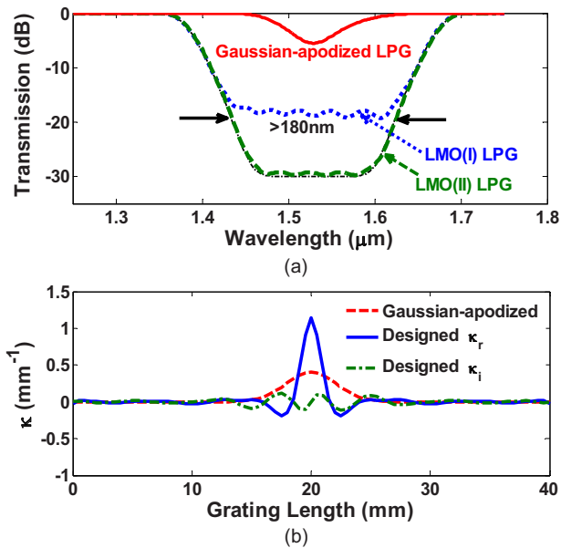
Fig. 2 (a) Transmission spectra of the designed UBLPGs. The dotted line is LMO(I) method using linear scale, and the dashed line is LMO(II) method with decibel scale. (b). Real ( \kappa_r ) and imaginary ( \kappa_i ) parts of the designed coupling coefficients of UBLPG, with a grating length of 4 cm.
