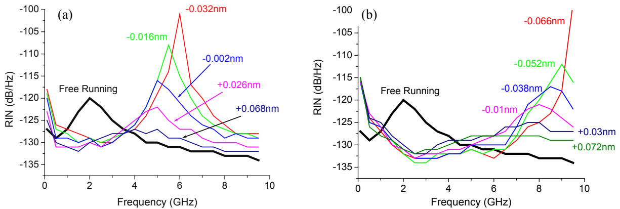
Figure 8. RIN spectra for (a) 10 dB-attenuated and (b) 5 dB-attenuated injection power. Free running RIN (thick curves) are shown as the reference. Note that the RIN peaks are prominent for the negative detuning cases for both injection powers. More than 10dB of RIN reduction is observed at 2 GHz and the reduction is relatively insensitive to the amount of detuning. For a higher injection power, the noise reduction is expected to be larger. Unfortunately, due to the thermally limited detector, the reduction is comparable in both cases studied here. The true RIN spectra can be obtained if a higher power VCSEL is available.
