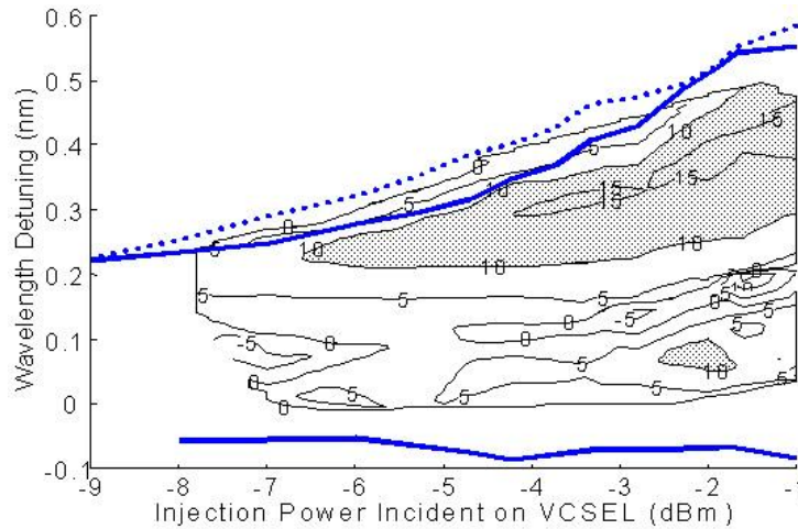
Figure 6. Third harmonic SFDR improvement. The shaded area corresponds to the case when improvement is larger than 10 dB. The plot shows an improvement of SFDR between 0.2 and 0.5 nm detuning. This large detuning tolerance makes the injection-locking technique attractive in a practical system.
