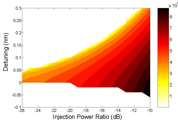
Figure 4. Simulated Arnold tongues of resonance frequency. The theory predicts the highest resonance frequency occurs at a high injection power and small detuning condition. Taking into account of the difference in the definition of the injection power between the experiment and the simulation, the tilted stripes in the figure will become more vertical. The overall trend predicted by the theory matches well to the experimental Arnold tongue.
