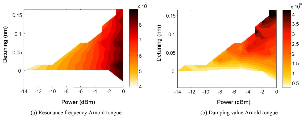
Figure 3. Experimental Arnold tongues of resonance frequency and damping. Generally speaking, a higher injection power is always desirable to improve the resonance frequency.
