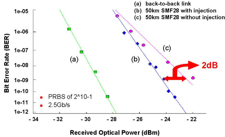
Figure 9. BER vs. received power for different conditions. Note the improvement after transmission through fiber when the VCSEL is injection-locked.
