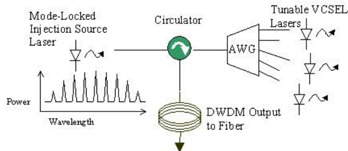
Figure 12. Proposed system architecture for uncooled injection-locked transmitters at different WDM grid. The master output is coupled into an AWG, which filters out only one wavelength component from the master, through a circulator. The filtered master field locks the uncooled tunable VCSELs to the ITU grid and improves their performances. The signal from each follower VCSEL is then coupled back to AWG, aggregated and sent to output fiber through the circulator.
