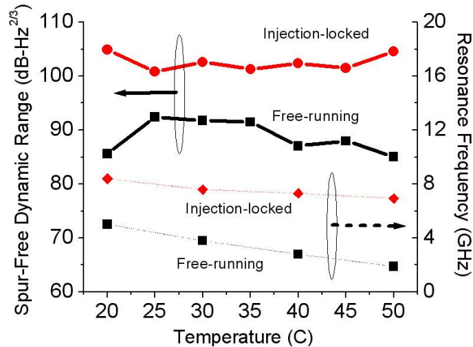
Figure 11. IMD3 SFDR and resonance frequency at various temperatures for both free running and injection locked cases. The modulation frequencies are at 990 MHz and 1 GHz for the SFDR measurement. The injection-locked SFDR is always better than the free running case provided a proper detuning is chosen. A constant enhancement of the resonance frequency is observed throughout the measured temperature range as well.
