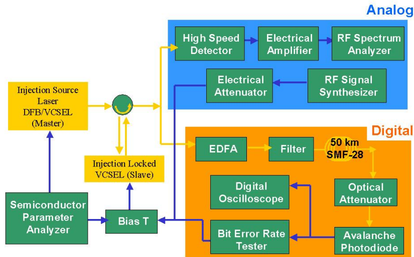
Figure 1. Injection locking setup for both digital and analog modulation.
