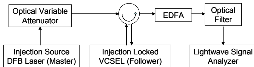
Figure 7. Experimental setup for RIN measurement.
