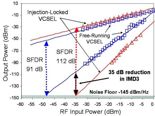
Figure 5. Third harmonic SFDR improvement with injection locking for an 1 GHz single-tone modulated VCSEL at 1538.4 nm. The incident DFB power is around -4 dBm with a detuning of +0.24 nm. SFDR is calculated with a RIN-limited system noise floor of -145 dBm/Hz. The increase in the fundamental tone accompanied with a decrease in the 3rd order harmonic distortion power enhanced the SFDR from 91 dB-Hz 2/3 to 112 dB-Hz 2/3 .
