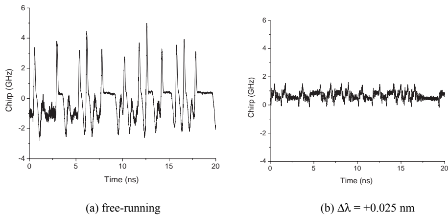
Figure 10. Chirp of the modulated VCSEL for the cases of free running and injection locked. The transient chirp, \sim 7.8 GHz, dominates in the free running case. In (b), the VCSEL is locked to 8 dBm, +0.025 nm detuned DFB. Both the transient and adiabatic chirp is reduced compared to its free running case.
