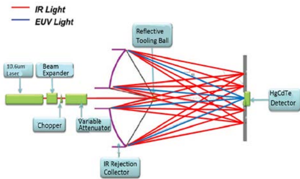
Fig. 6 Schematic of new type filter
