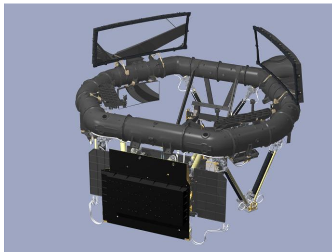
Fig. 1. The GAIA Payload Module features “all in SiC” architecture Proc. of SPIE Vol. 10565 105652C-2
