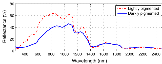
Fig. 1 Reflectance spectra for lightly and darkly pigmented skin specimens provided by Cooksey and Allen 6 and Jacquez et al., 7,8 respectively.
