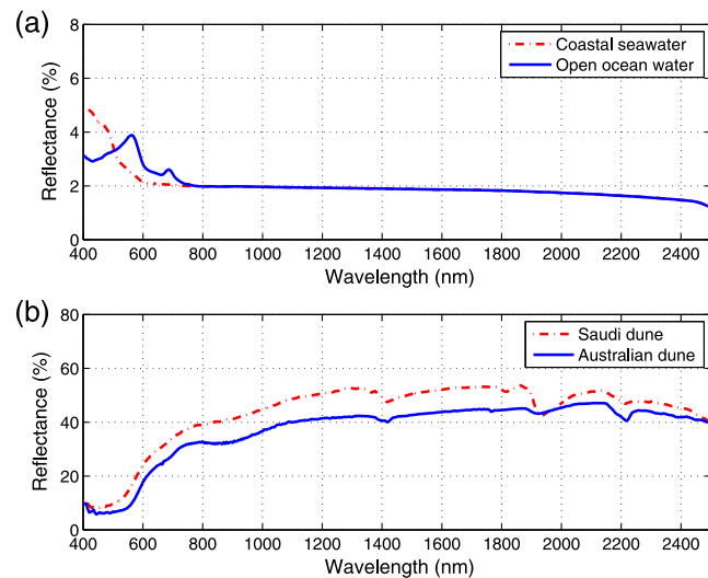
Fig. 2 Reflectance spectra for sample materials characterized by the absence of prominent features at the near-infrared (NIR) wavelengths of interest. (a) Ocean water samples. 9 (b) Desert (dune) sand samples. 10
