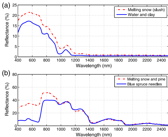
Fig. 3 Reflectance spectra 9 for sample materials characterized by the presence of prominent features at the NIR wavelengths of interest. (a) Melting snow (slush) and water mixed with clay (1.67 g/L). (b) Melting snow mixed with forest vegetation (pinyon pine), and fresh blue spruce needles.
