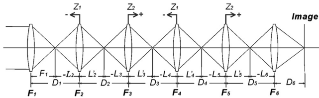
Fig. 3 General six-component zoom system.
