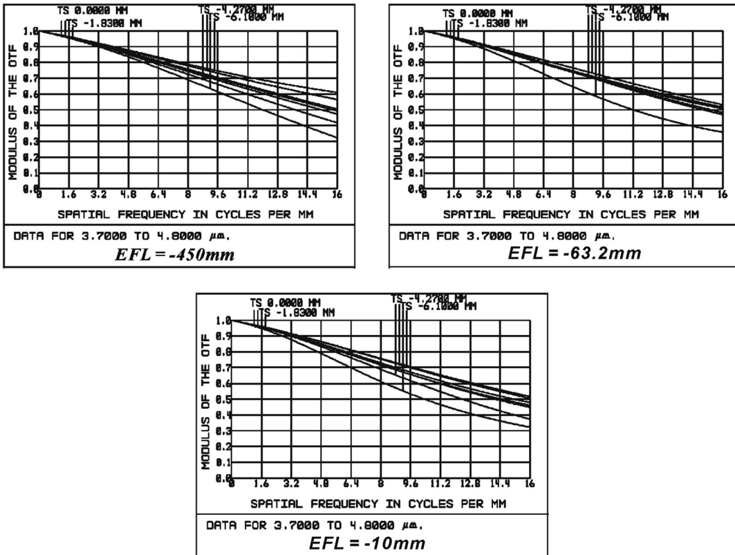
Fig. 6 MTF curves of the system at three zoom positions.
