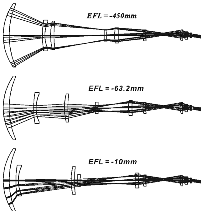
Fig. 4 Layouts of the actual system at three zoom positions.
