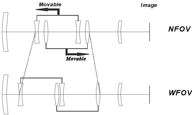
Fig. 2 Six-component mechanically compensated zoom system.
