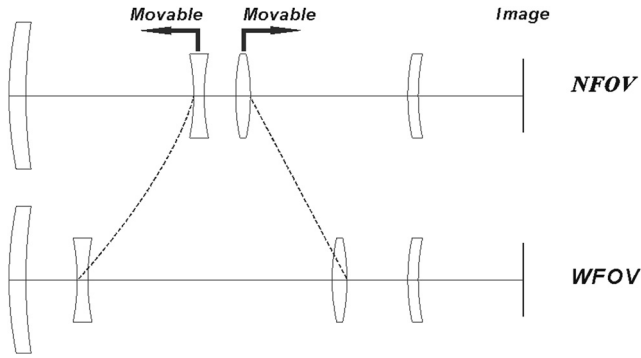
Fig. 1 Four-component mechanically compensated zoom system.
