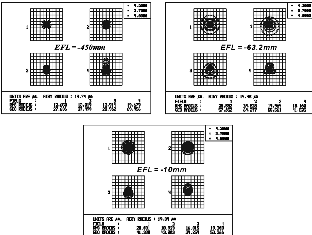
Fig. 7 Spot diagrams of the system at three zoom positions.
