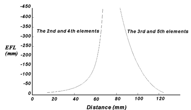
Fig. 5 The zoom paths of the actual system.
