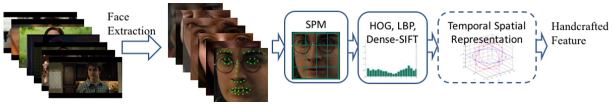
Fig. 4 Pipeline of handcrafted features extraction. The dashed box means that the temporal–spatial representation is only used for AFEW dataset.
