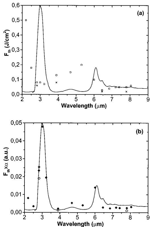
Fig. 6 Dependency of denaturation threshold F_{th} (in J/cm^2 ) as a function of wavelength \lambda (in \mu m ); the plotted solid curve is the absorption spectrum for cartilage in arbitrary units: (a) F_{th} versus \lambda ; ( \square ) cartilage, ( * ) cornea; and (b) composition \alpha F_{th} versus \lambda ; ( \bullet ) cartilage and ( \circ ) cornea.
