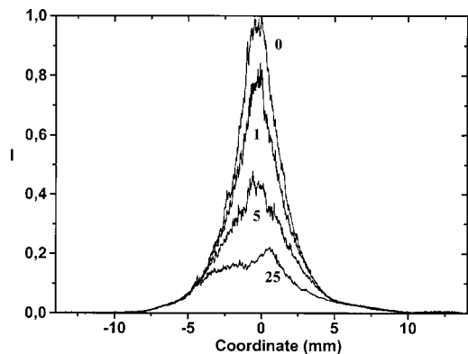
Fig. 2 The spatial distribution of a probe beam at the plane of a photodiode array (magnification \times 2.8 ) and its alternations by cartilage irradiated by FEL. The numbers refer to the duration of the irradiation (in seconds); FEL wavelength \lambda = 8.5 \mu\text{m} , pulse radiant exposure F = 0.23 \text{ J/cm}^2 , f = 20 \text{ Hz} . I is the intensity of the visible scattered light in arbitrary units, and Coordinate is the position on the photodiode array in millimeters.
